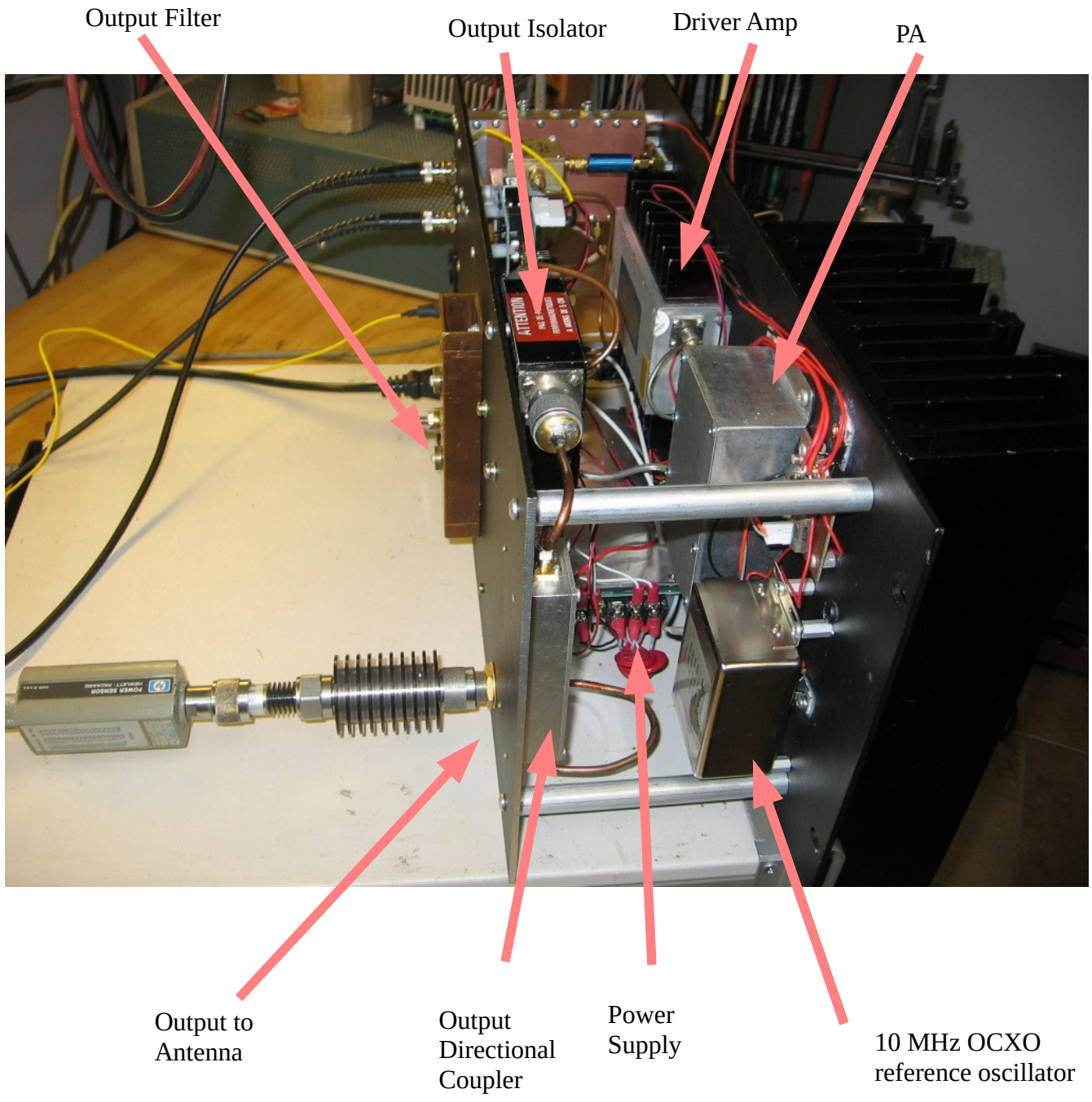
Figure 2: Beacon internal view, power amplifier (PA) view.
