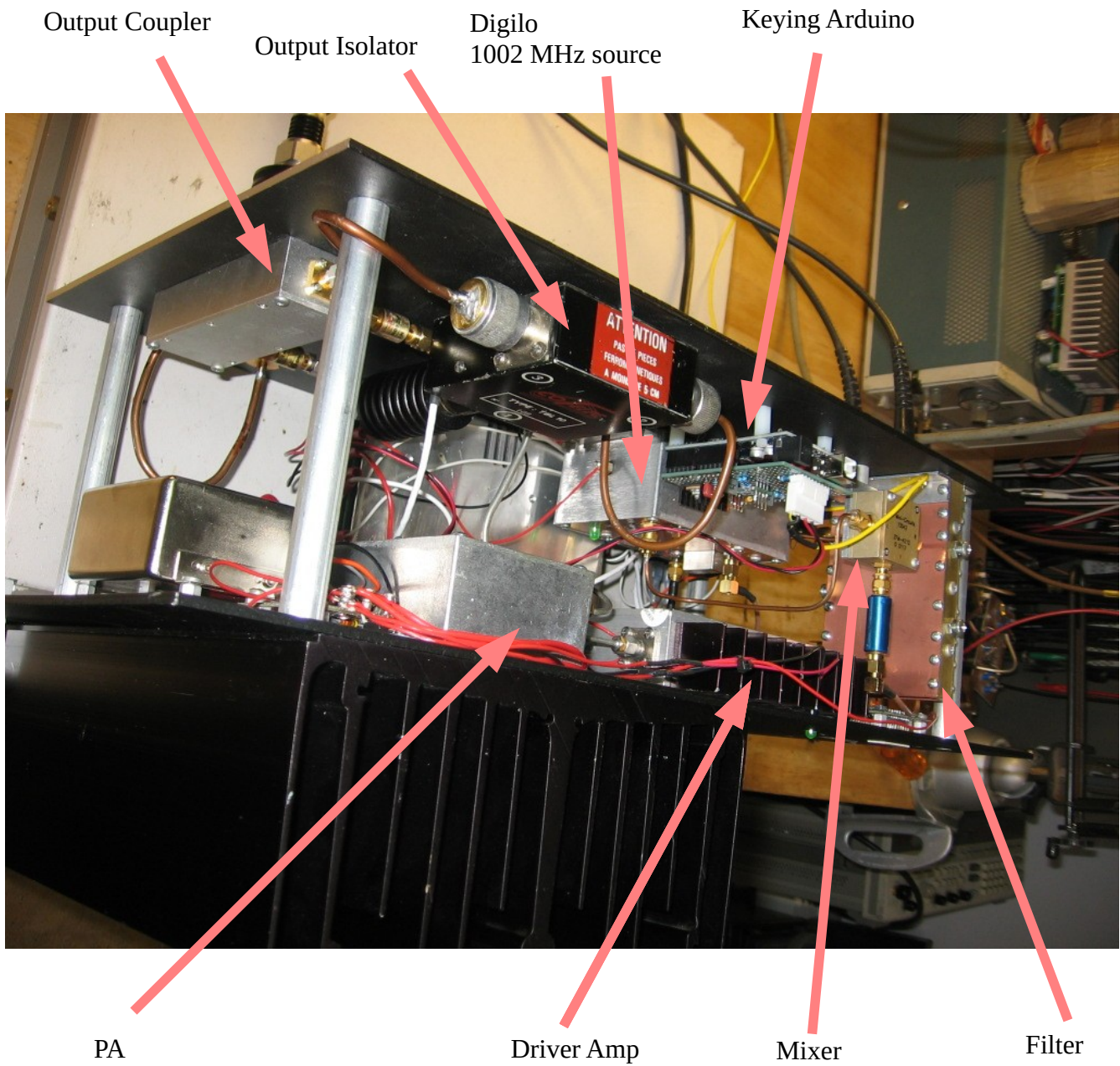
Figure 4: Beacon internal view, above.
