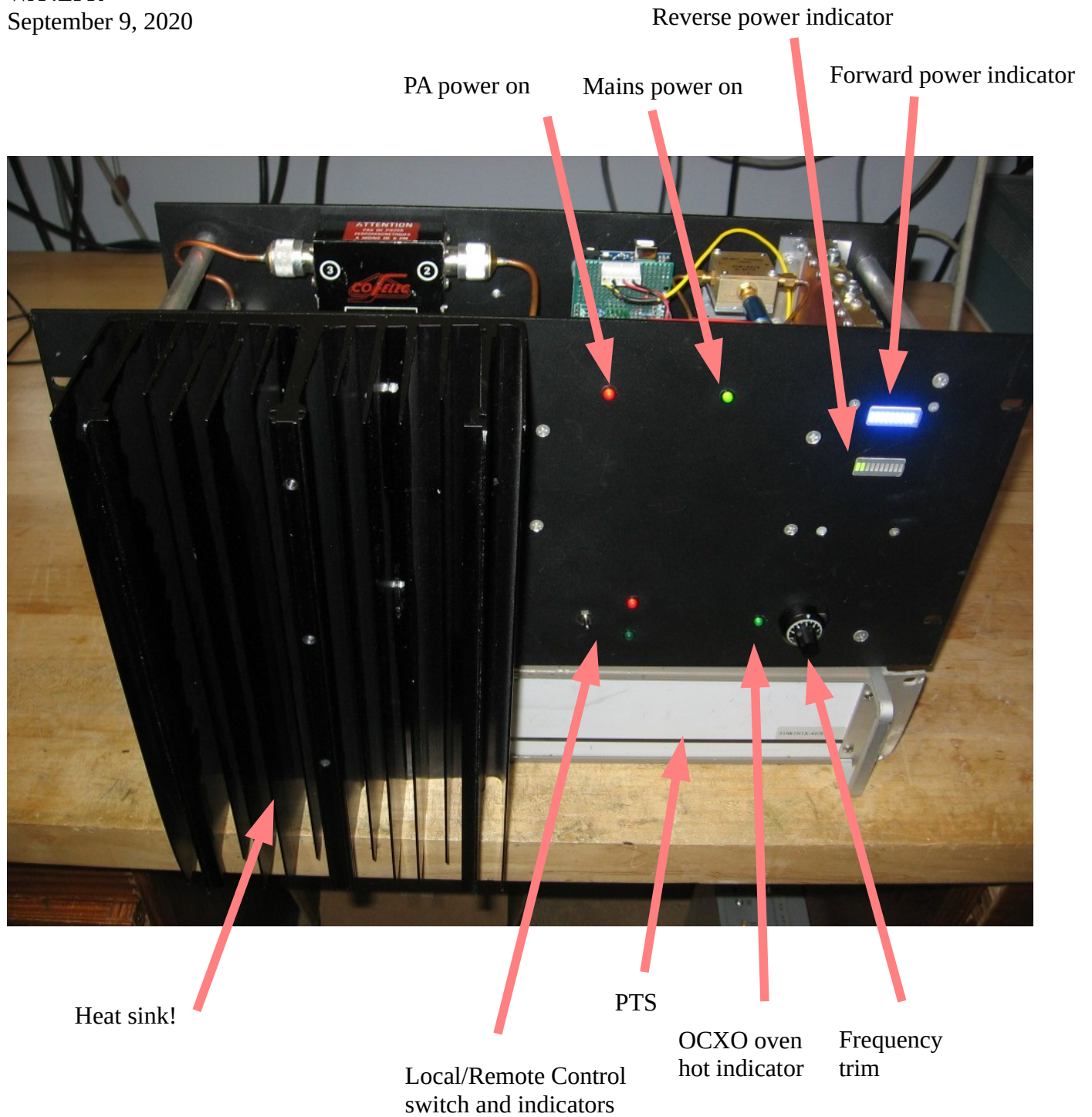
Figure 1: Beacon front panel.
