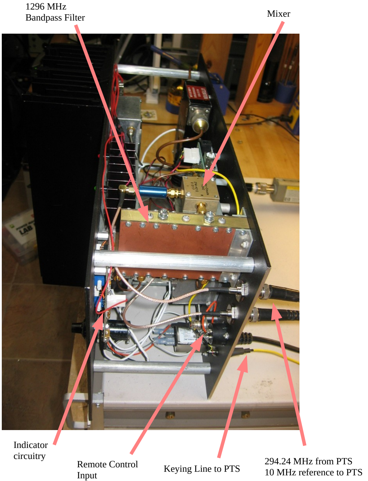
Figure 3: Beacon internal view, filter end.
